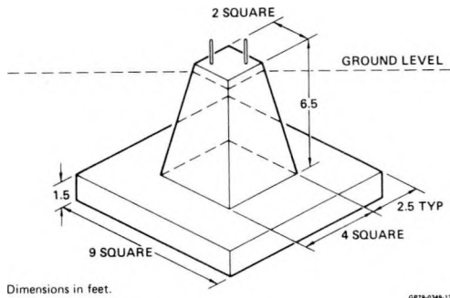
FIGURE 19 FOUNDATION PIER
