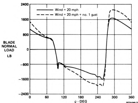
FIGURE 11 BLADE AERODYNAMIC NORMAL LOAD 6.0 ROTOR DESIGN
