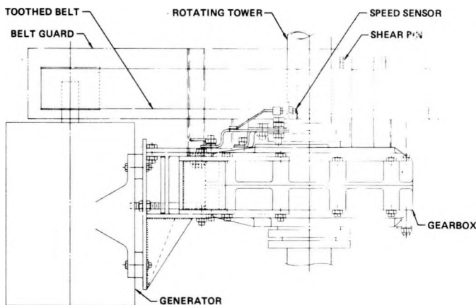
FIGURE 36 ELECTRICAL DRIVE SYSTEM ASSEMBLY Side View
