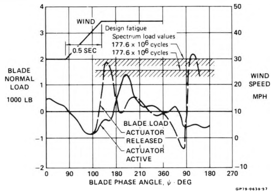
FIGURE 24 BLADE LOADS DUE TO SEVERE GUST
