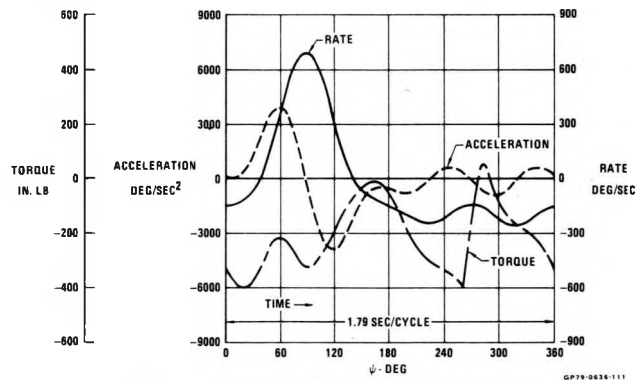
FIGURE 30 BLADE ACTUATOR REQUIREMENTS 40 MPH
