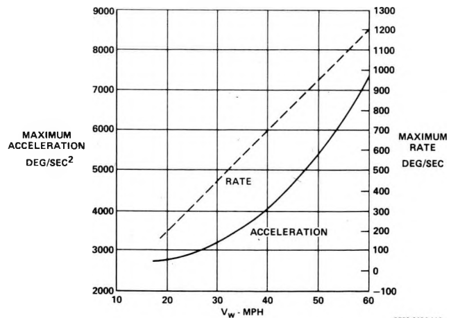
FIGURE 31 BLADE ACTUATOR MAXIMUM RATE AND ACCELERATION
