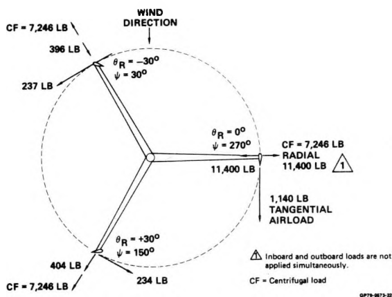
FIGURE 10 GIROMILL ULTIMATE DESIGN LOAD Condition 1
