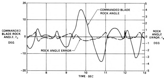
FIGURE 27 BLADE 1 ROCK ANGLE AND ROCK ANGLE ERROR Below-Rated-Power Wind Gust
