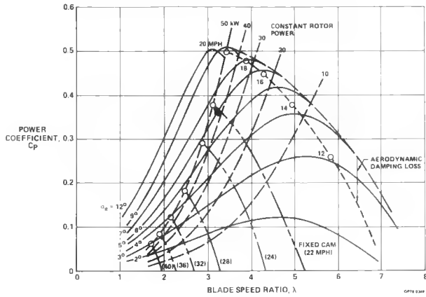
FIGURE 5 GIROMILL CONTROL PERFORMANCE
