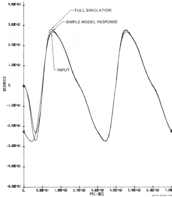
FIGURE 32 ACTUATOR MODEL COMPARISON 40 MPH
