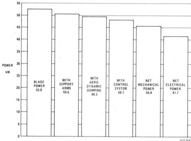
FIGURE 6 POWER OUTPUT BREAKDOWN 20 MPH Wind
