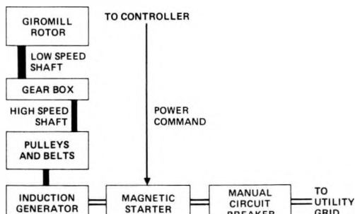
FIGURE 37 BLOCK DIAGRAM OF GIROMILL ELECTRICAL OUTPUT POWER FOR OPERATION WITH A LARGE UTILITY GRID
