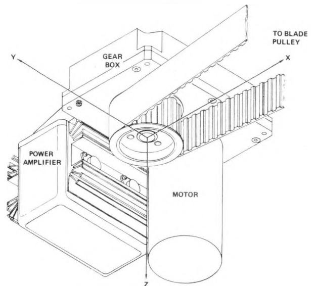
FIGURE 35 BLADE ACTUATOR ASSEMBLY
