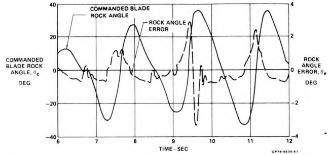
FIGURE 28 BLADE 1 ROCK ANGLE AND ROCK ANGLE ERROR Above-Rated-Power Wind Gust
