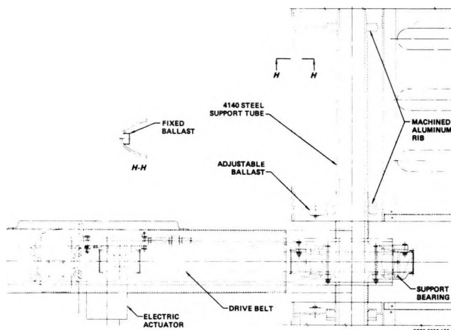
FIGURE 13 BLADE GENERAL ARRANGEMENT
