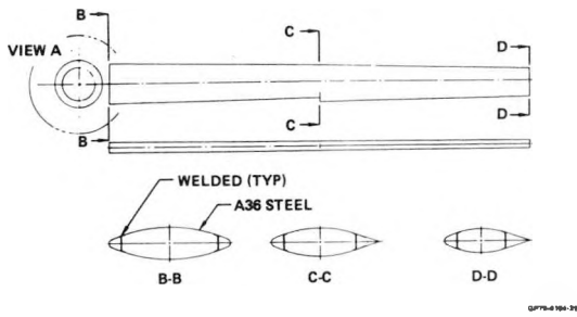
FIGURE 14 GENERAL ARRANGEMENT SUPPORT ARM
