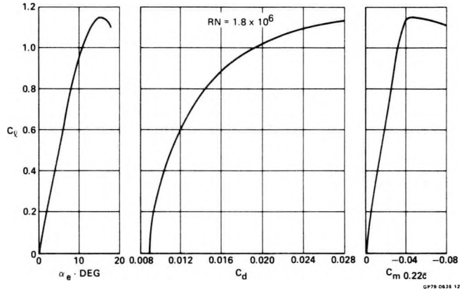
FIGURE 3 BLADE AERODYNAMIC CHARACTERISTICS NACA 0013 With Trailing Edge Modification
