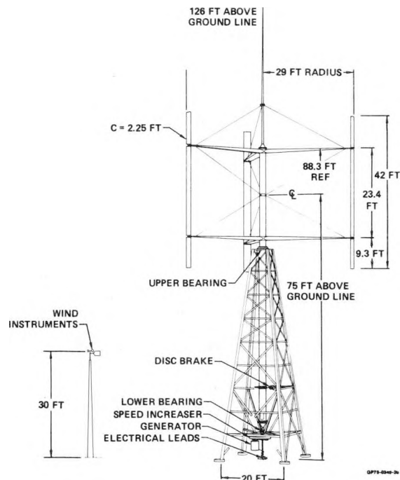
FIGURE 1 SELECTED CONFIGURATION
