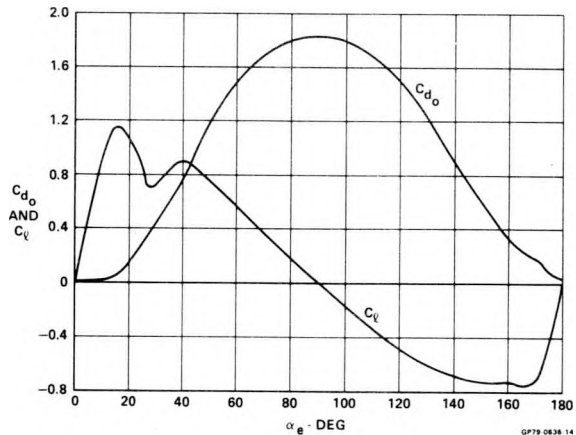
FIGURE 4 GIROMILL BLADE AERODYNAMIC CHARACTERISTICS
