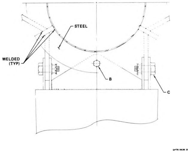
FIGURE 15 ARM/TOWER ATTACHMENT
