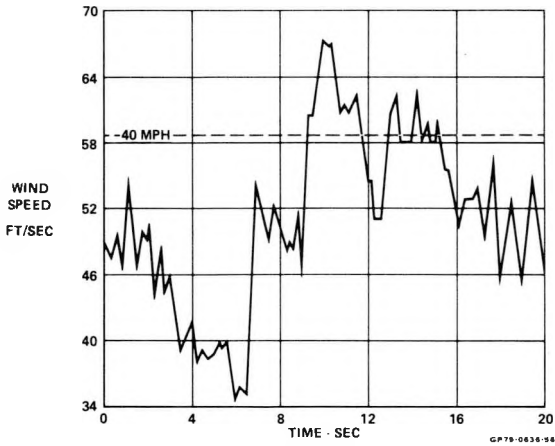
FIGURE 26 ABOVE-RATED-POWER WIND GUST
