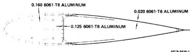
FIGURE 12 BLADE CROSS-SECTION
