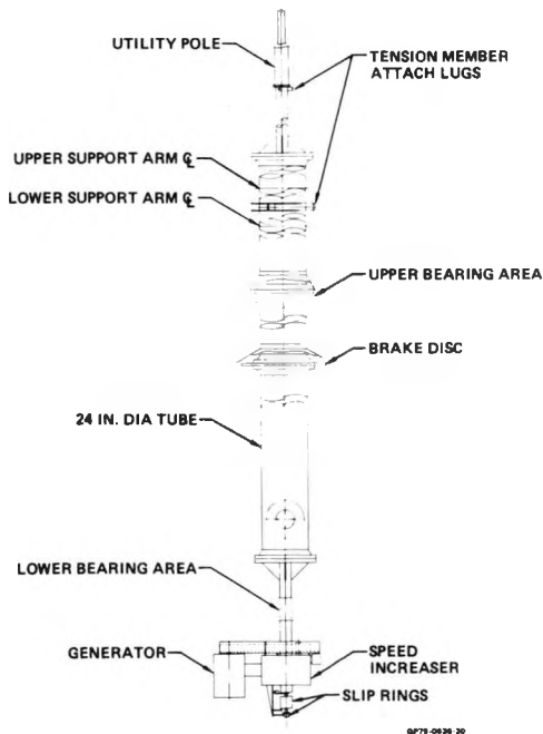
FIGURE 16 ROTATING TOWER
