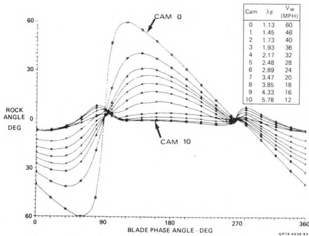
FIGURE 33 PROGRAMMED ROCK ANGLE PROFILES
