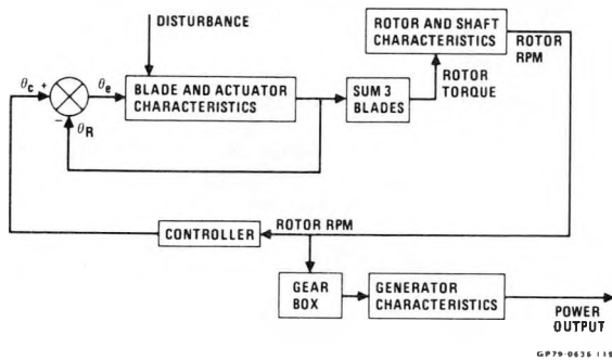
FIGURE 22 STEADY STATE LINEARIZED CONTROL SYSTEM REPRESENTATION
