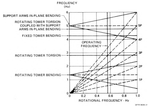
FIGURE 21 STRUCTURAL FREQUENCIES VS ROTATION Fixed Coordinate System
