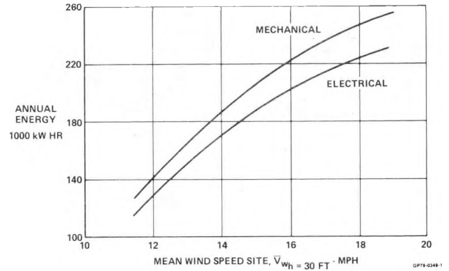
FIGURE 7 ANNUAL ENERGY
