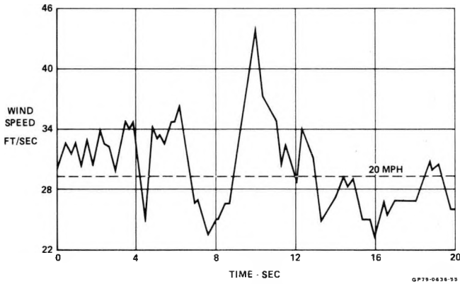
FIGURE 25 BELOW-RATED-POWER WIND GUST
