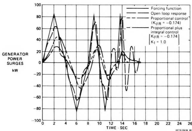
FIGURE 23 STEADY STATE LINEARIZED CONTROL TIME RESPONSES
