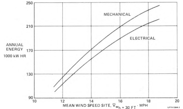
FIGURE 8 ANNUAL ENERGY
