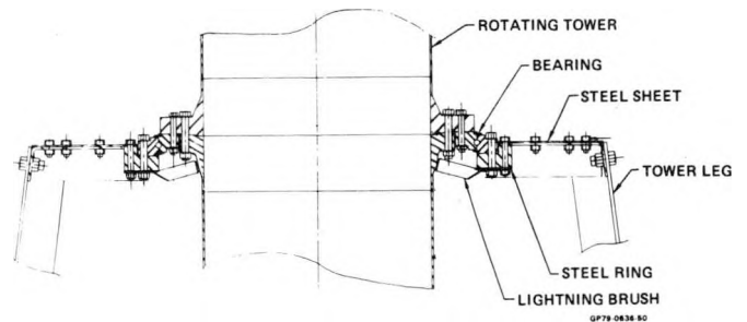
FIGURE 18 UPPER BEARING MOUNTING Side View
